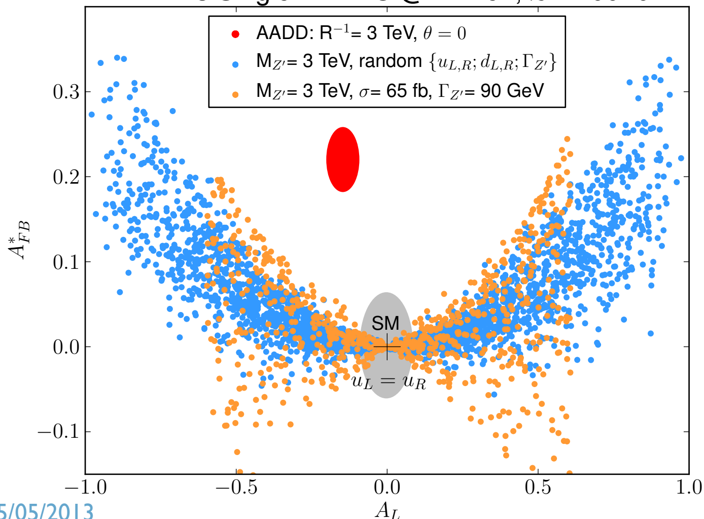
AADD vs Single Z' : LHC @ 14 TeV, \mathcal{L} = 100 \text{ fb}^{-1}
