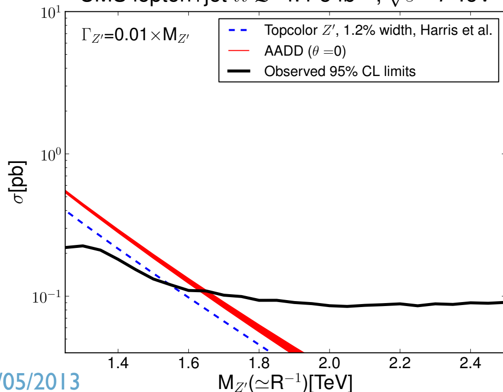
CMS lepton+jet t\bar{t} \mathcal{L} = 4.4\text{-}5 \text{ fb}^{-1} ; \sqrt{s} = 7 TeV
