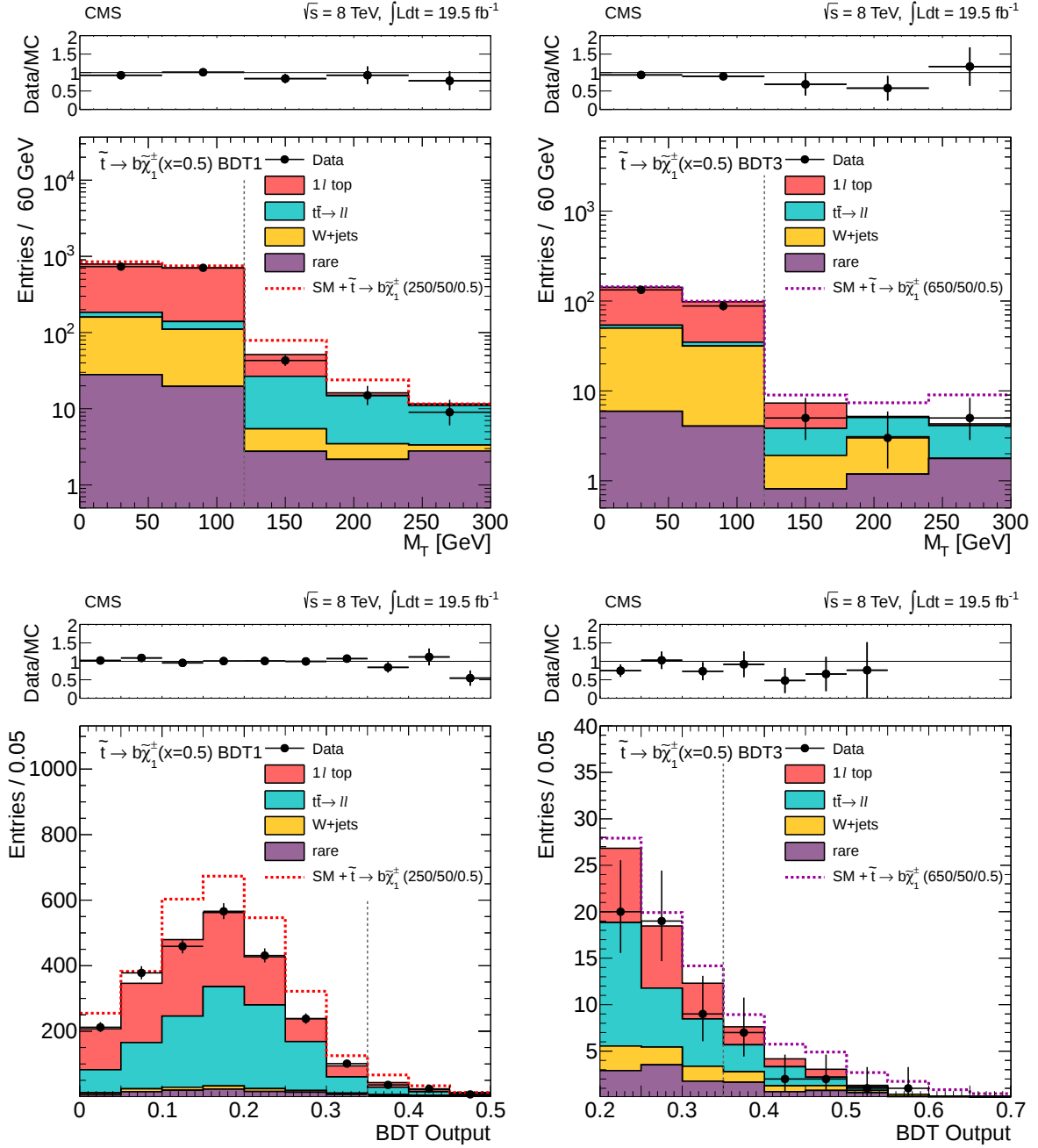
Figure 9: Comparison of the M_T (top) and BDT output (bottom) distributions in data and MC simulation for events satisfying the loosest (left) and tightest (right) \tilde{t} \rightarrow b\tilde{\chi}_1^+ BDT signal region requirements for x = 0.5 and with an on-shell W boson. For the M_T plots, the BDT output signal region requirement is imposed; For the BDT plots, the M_T > 120 GeV requirement is imposed. The distributions for the \tilde{t} \rightarrow b\tilde{\chi}_1^+ model with m_{\tilde{t}} = 250 GeV (left) and m_{\tilde{t}} = 650 GeV (right) for m_{\tilde{\chi}_1^0} = 50 GeV and x = 0.5 , are overlaid. The vertical dashed line indicates the corresponding signal region requirement.
