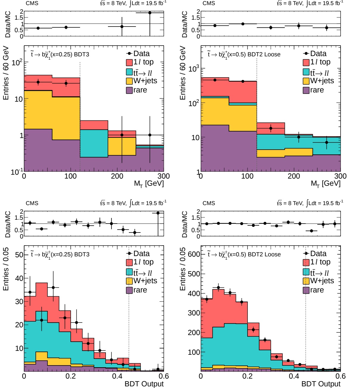
Figure 16: Comparison of the M_T (top) and BDT-output (bottom) distributions in data vs. MC for events satisfying the BDT3 \tilde{t} \rightarrow b\tilde{\chi}_1^+ x = 0.25 (left) and BDT2 loose \tilde{t} \rightarrow b\tilde{\chi}_1^+ x = 0.5 (right) BDT signal region requirements. For the M_T plots, the BDT-output signal region requirement is imposed; for the BDT plots, the M_T > 120 GeV requirement is imposed. The vertical dashed lines indicate the lower edge of the corresponding signal region requirement.
