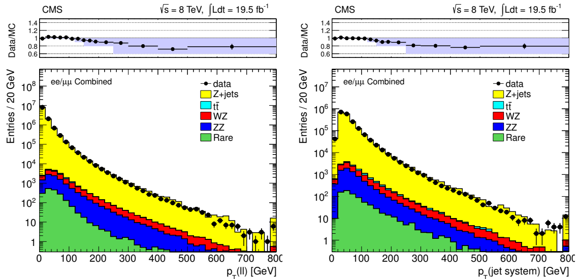
Figure 24: Comparison of data to MC predictions for the dilepton p_T (left) and jet recoil system p_T (right) in Z + \text{jets} events. The MC prediction is normalized to the total data yield. The data/MC ratio is also shown. The shaded band is centered on the weight values. The width of the band indicates the associated systematic uncertainty.
