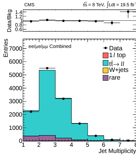
Figure 5: Comparison of the jet multiplicity distributions in data and MC simulation in the sample dominated by t\bar{t} \rightarrow \ell\ell events.
