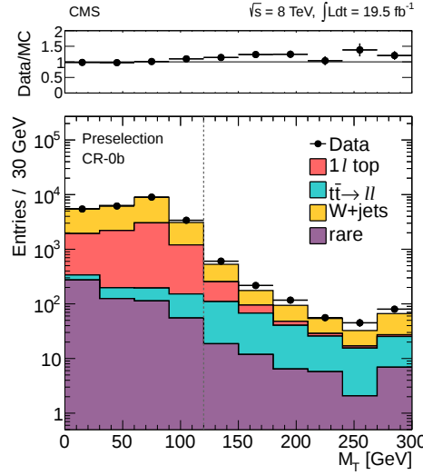
Figure 7: Comparison of data and MC simulation for the M_T distribution in the CR-0b control region, after the preselection. The M_T tail is underestimated by the simulation. A scale factor derived from this control region is used to correct the predictions of the W + \text{jets} and single-lepton-top-quark backgrounds.
