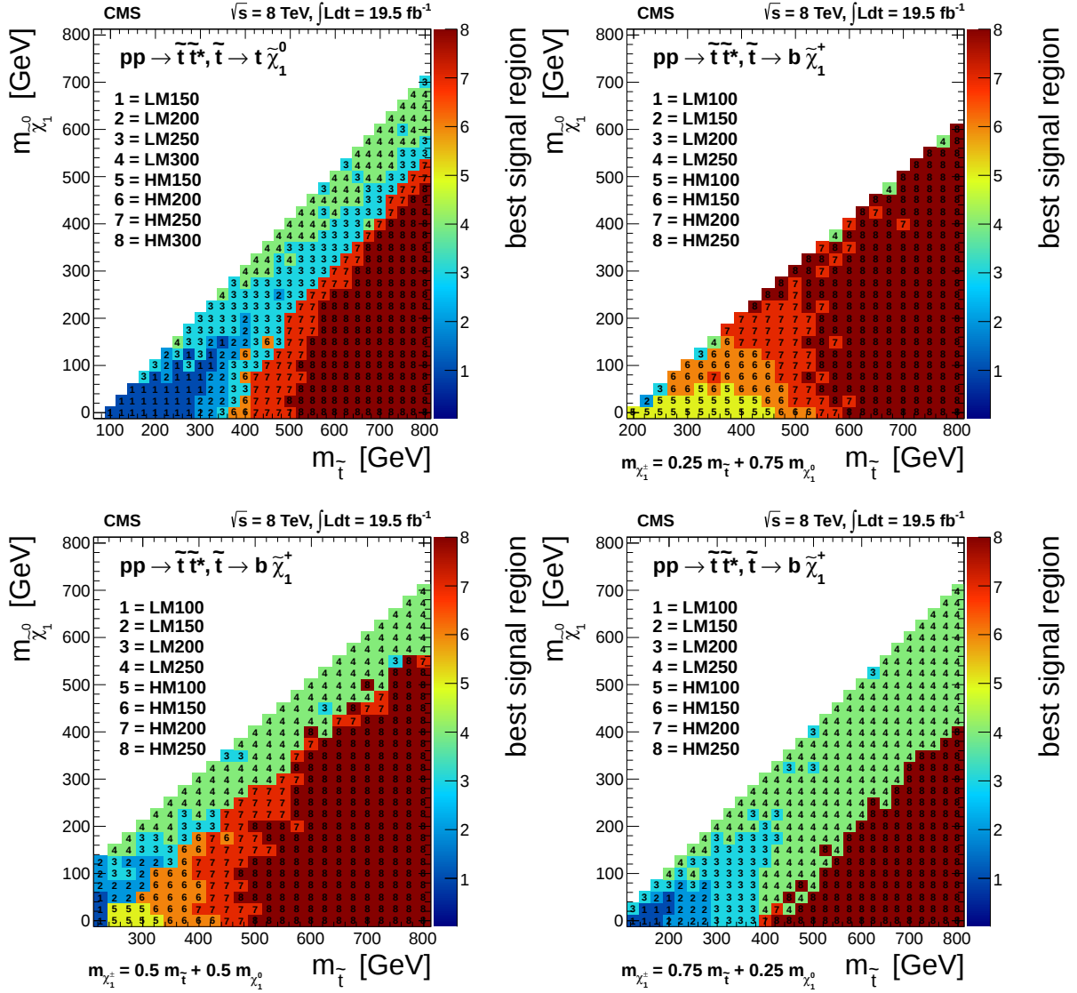
Figure 22: The most sensitive signal region in the m_{\tilde{\chi}_1^0} vs. m_{\tilde{t}} parameter space in the cut-based analysis, for the (top left) \tilde{t} \rightarrow \tilde{\chi}_1^0 model, and the \tilde{t} \rightarrow b \tilde{\chi}_1^+ model with chargino mass parameter (top right) x = 0.25 , (bottom left) 0.5, and (bottom right) 0.75. LM and HM refer to low \Delta M and high \Delta M , respectively, and the number indicates the E_T^{\text{miss}} requirement.
