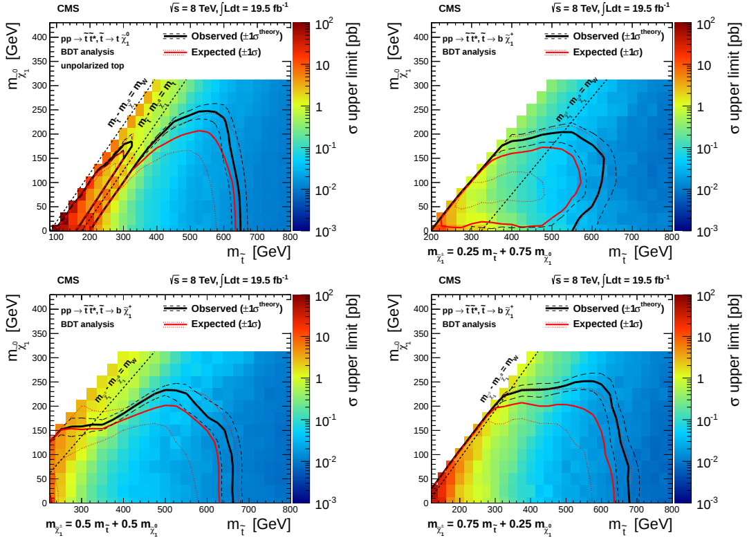
Figure 10: Interpretations using the primary results from the BDT method for the (top left) \tilde{t} \rightarrow t\tilde{\chi}_1^0 model, and for the \tilde{t} \rightarrow b\tilde{\chi}_1^+ model with chargino mass parameter (top right) x = 0.25 , (bottom left) 0.5, and (bottom right) 0.75. The color scale indicates the observed cross section upper limit. The observed, median expected, and \pm 1 standard deviation ( \sigma ) expected 95% CL exclusion contours are indicated.
