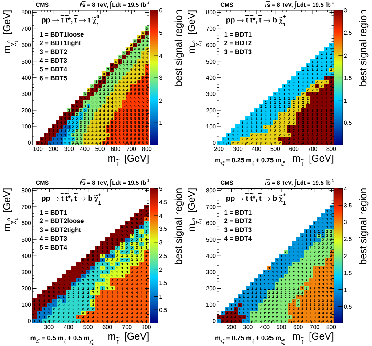
Figure 21: The most sensitive signal region in the m_{\tilde{\chi}_1^0} vs. m_{\tilde{t}} parameter space in the BDT analysis, for the (top left) \tilde{t} \rightarrow \tilde{\chi}_1^0 model, and the \tilde{t} \rightarrow b\tilde{\chi}_1^+ model with chargino mass parameter (top right) x = 0.25 , (bottom left) 0.5 , and (bottom right) 0.75 . The number indicates the BDT training region.
