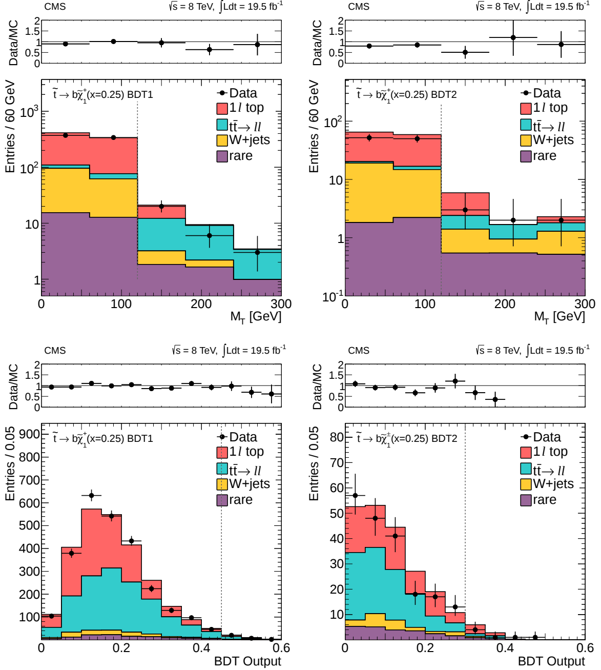
Figure 15: Comparison of the M_T (top) and BDT-output (bottom) distributions in data vs. MC for events satisfying the BDT1 (left) and BDT2 (right) \tilde{t} \rightarrow b\tilde{\chi}_1^+ x = 0.25 BDT signal region requirements. For the M_T plots, the BDT-output signal region requirement is imposed; for the BDT plots, the M_T > 120 GeV requirement is imposed. The vertical dashed lines indicate the lower edge of the corresponding signal region requirement.
