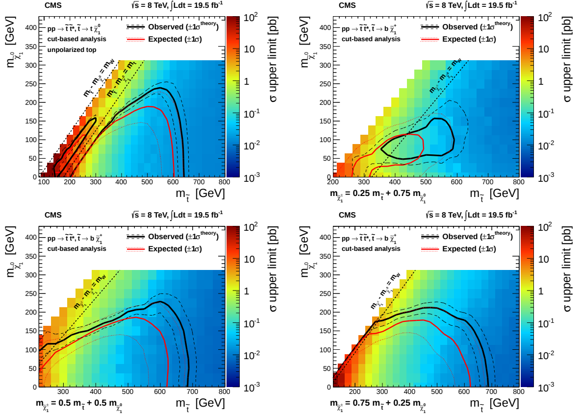
Figure 20: Interpretations based on the results of the cut-based analysis, for the (top left) \tilde{t} \rightarrow t\tilde{\chi}_1^0 model, and the \tilde{t} \rightarrow b\tilde{\chi}^+ model with chargino mass parameter (top right) x = 0.25 , (bottom left) 0.5, and (bottom right) 0.75. The color scale indicates the observed cross section upper limit. The observed (solid black), median expected (solid red), and \pm 1\sigma expected (dotted red) 95% CL exclusion contours are indicated. The variations in the excluded region due to \pm 1\sigma uncertainty of the theoretical prediction of the cross section for top-squark pair production are also indicated.
