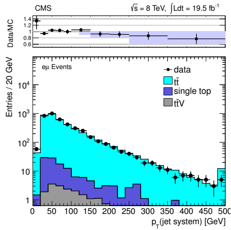
Figure 25: Comparison of data to MC prediction for the jet recoil system p_T in t\bar{t} events. The MC prediction is normalized to the total data yield. The ratio of data/MC is also shown. The shaded band shows the weights derived for MC simulation and the variation to assess systematic uncertainties.
