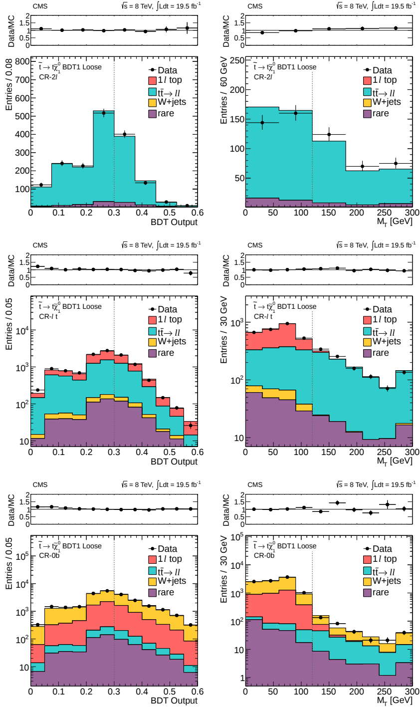
Figure 6: Comparison of data and MC simulation in the CR-2 \ell (top row), CR- \ell t (middle row), and CR-0b (bottom row) control regions, for the output distribution of the \tilde{t} \rightarrow t\tilde{\chi}_1^0 model BDT1 (left), and for the corresponding M_T distribution (right) after the signal-like requirement on the BDT1 output (“BDT1 Loose”, indicated by the dashed lines in the left plots). The dashed lines in the right plots indicate the M_T > 120 GeV selection requirement. For the CR-0b plot, the scale factors are applied to the MC distribution in the M_T tail. For all plots, the last bin contains the overflow.
