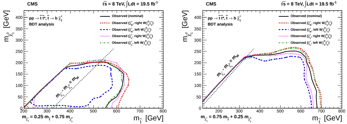
Figure 23: The observed 95% CL excluded regions for the \tilde{t} \rightarrow b\tilde{\chi}^+ model with x = 0.25 (left) and 0.75 (right) for the nominal scenario in the signal model, right- vs. left-handed charginos ( \tilde{\chi}_R^\pm and \tilde{\chi}_L^\pm , respectively), and right- vs. left-handed W\tilde{\chi}_1^0 \tilde{\chi}_1^\pm couplings.
