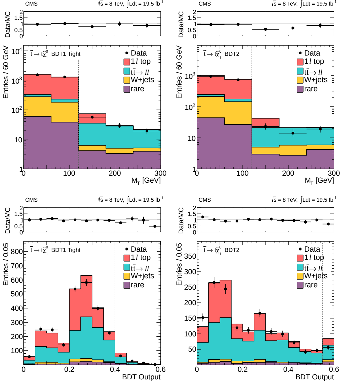
Figure 13: Comparison of the M_T (top) and BDT-output (bottom) distributions in data vs. MC for events satisfying the BDT1 tight (left) and BDT2 (right) \tilde{t} \rightarrow t\tilde{\chi}_1^0 BDT signal region requirements. For the M_T plots, the BDT-output signal region requirement is imposed; for the BDT plots, the M_T > 120 GeV requirement is imposed. The vertical dashed lines indicate the lower edge of the corresponding signal region requirement.
