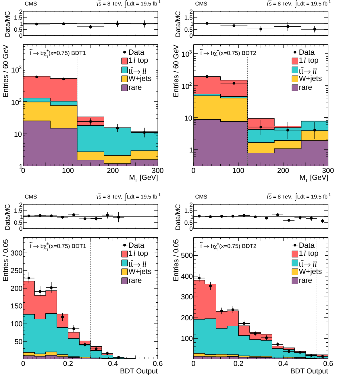
Figure 18: Comparison of the M_T (top) and BDT-output (bottom) distributions in data vs. MC for events satisfying the BDT1 (left) and BDT2 (right) \tilde{t} \rightarrow b\tilde{\chi}_1^+ x = 0.75 BDT signal region requirements. For the M_T plots, the BDT-output signal region requirement is imposed; for the BDT plots, the M_T > 120 GeV requirement is imposed. The vertical dashed lines indicate the lower edge of the corresponding signal region requirement.
