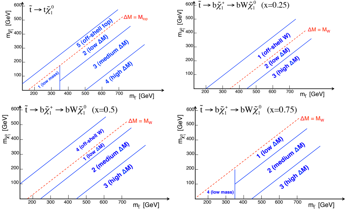
Figure 3: The regions used to train the BDTs, in the m_{\tilde{\chi}_1^0} vs. m_{\tilde{t}} parameter space, for the \tilde{t} \rightarrow t\tilde{\chi}_1^0 scenario (top left), and for the \tilde{t} \rightarrow b\tilde{\chi}_1^+ \rightarrow bW\tilde{\chi}_1^0 ( x=0.25 ) (top right), 0.5 (bottom left), and 0.75 (bottom right) scenarios. The dashed lines correspond to \Delta M \equiv m_{\tilde{t}} - m_{\tilde{\chi}_1^0} = M_{\text{top}} for \tilde{t} \rightarrow t\tilde{\chi}_1^0 , and \Delta M \equiv m_{\tilde{\chi}_1^+} - m_{\tilde{\chi}_1^0} = M_W for \tilde{t} \rightarrow b\tilde{\chi}_1^+ .
