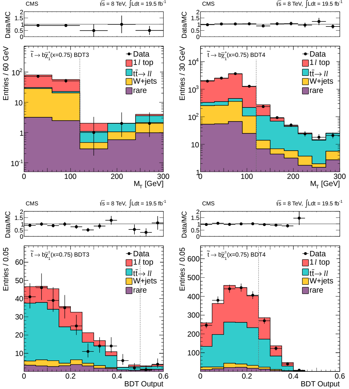
Figure 19: Comparison of the M_T (top) and BDT-output (bottom) distributions in data vs. MC for events satisfying the BDT3 (left) and BDT4 (right) \tilde{t} \rightarrow b\tilde{\chi}_1^+ x = 0.75 BDT signal region requirements. For the M_T plots, the BDT-output signal region requirement is imposed; for the BDT plots, the M_T > 120 GeV requirement is imposed. The vertical dashed lines indicate the lower edge of the corresponding signal region requirement.
