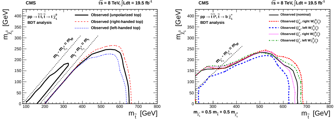
Figure 11: Left: the observed 95% CL excluded regions for the \tilde{t} \rightarrow t\tilde{\chi}_1^0 model for the case of unpolarized, right-handed, and left-handed top quarks. Right: the observed 95% CL excluded regions for the \tilde{t} \rightarrow b\tilde{\chi}_1^+ model with x = 0.5 for the nominal scenario, right- vs. left-handed charginos ( \tilde{\chi}_R^\pm and \tilde{\chi}_L^\pm , respectively), and right- vs. left-handed W\tilde{\chi}_1^\pm couplings.
