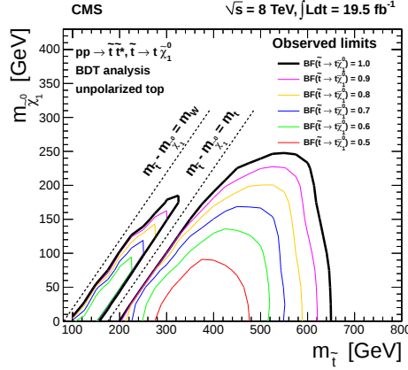
Figure 12: The observed 95% CL excluded regions as a function of the assumed branching fraction for the \tilde{t} \rightarrow t\tilde{\chi}_1^0 decay mode. The results are based on the assumption that the search has no acceptance for top-squark pair events if one of the top squarks decays in a different mode. See text for details.
