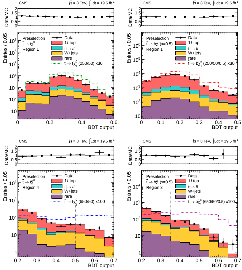
Figure 4: Comparison of data and MC simulation for the BDT output of the \tilde{t} \rightarrow t\tilde{\chi}_1^0 scenario in training region 1 (top left) and region 4 (bottom left), and for the \tilde{t} \rightarrow b\tilde{\chi}_1^+ scenario with x = 0.5 in training region 1 (top right) and region 3 (bottom right). The last bins contain the overflow. Only the event preselection is applied. Events in the signal regions are further selected by requiring M_T > 120 GeV and by applying BDT requirements as indicated by the vertical dashed lines. For the top row of plots, distributions for the \tilde{t} \rightarrow t\tilde{\chi}_1^0 model (left) and for the \tilde{t} \rightarrow b\tilde{\chi}_1^+ model with x = 0.5 (right) for m_{\tilde{t}} = 250 GeV and m_{\tilde{\chi}_1^0} = 50 GeV, scaled by a factor of 30, are overlayed. For the bottom row, distributions for the \tilde{t} \rightarrow t\tilde{\chi}_1^0 model (left) and for the \tilde{t} \rightarrow b\tilde{\chi}_1^+ model with x = 0.5 (right) for m_{\tilde{t}} = 650 GeV and m_{\tilde{\chi}_1^0} = 50 GeV, scaled by a factor of 100, are shown.
