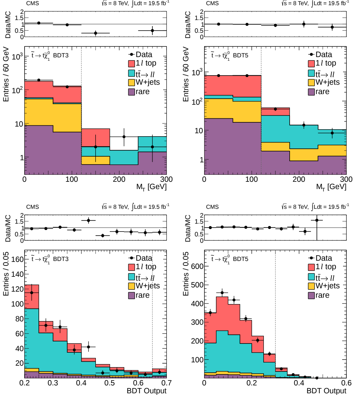
Figure 14: Comparison of the M_T (top) and BDT-output (bottom) distributions in data vs. MC for events satisfying the BDT3 (left) and BDT5 (right) \tilde{t} \rightarrow t\tilde{\chi}_1^0 BDT signal region requirements. For the M_T plots, the BDT-output signal region requirement is imposed; for the BDT plots, the M_T > 120 GeV requirement is imposed. The vertical dashed lines indicate the lower edge of the corresponding signal region requirement.
