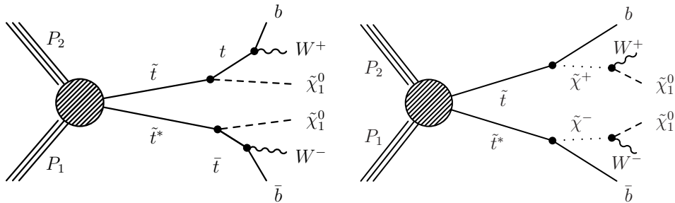
Figure 1: Diagram for top-squark pair production for the \tilde{t} \rightarrow t\tilde{\chi}_1^0 \rightarrow bW\tilde{\chi}_1^0 decay mode (left) and the \tilde{t} \rightarrow b\tilde{\chi}^+ \rightarrow bW\tilde{\chi}_1^0 decay mode (right).
