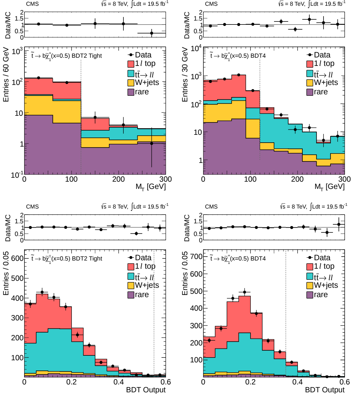
Figure 17: Comparison of the M_T (top) and BDT-output (bottom) distributions in data vs. MC for events satisfying the BDT2 tight (left) and BDT4 (right) \tilde{t} \rightarrow b\tilde{\chi}_1^+ x = 0.5 BDT signal region requirements. For the M_T plots, the BDT-output signal region requirement is imposed; for the BDT plots, the M_T > 120 GeV requirement is imposed. The vertical dashed lines indicate the lower edge of the corresponding signal region requirement.
