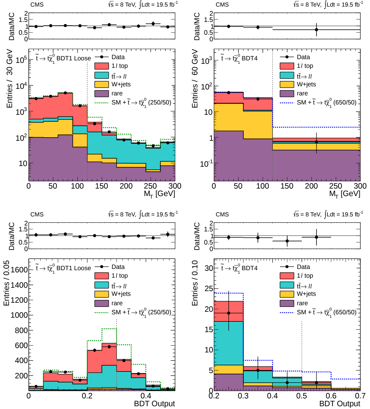
Figure 8: Comparison of the M_T (top) and BDT output (bottom) distributions in data and MC simulation for events satisfying the loosest (left) and tightest (right) \tilde{t} \rightarrow t\tilde{\chi}_1^0 BDT signal region requirements. For the M_T plots, the BDT output signal region requirement is imposed. For the BDT plots, the M_T > 120 GeV requirement is imposed. The distributions for the \tilde{t} \rightarrow t\tilde{\chi}_1^0 model with m_{\tilde{t}} = 250 GeV (left) and m_{\tilde{t}} = 650 GeV (right) for m_{\tilde{\chi}_1^0} = 50 GeV, are overlaid. The vertical dashed line indicates the corresponding signal region requirement. For the M_T distribution with the BDT4 requirement (upper right), the bin to the right of the vertical line contains all events with M_T > 120 GeV, and has been scaled by a factor of 1/3 to indicate the number of events per 60 GeV.
